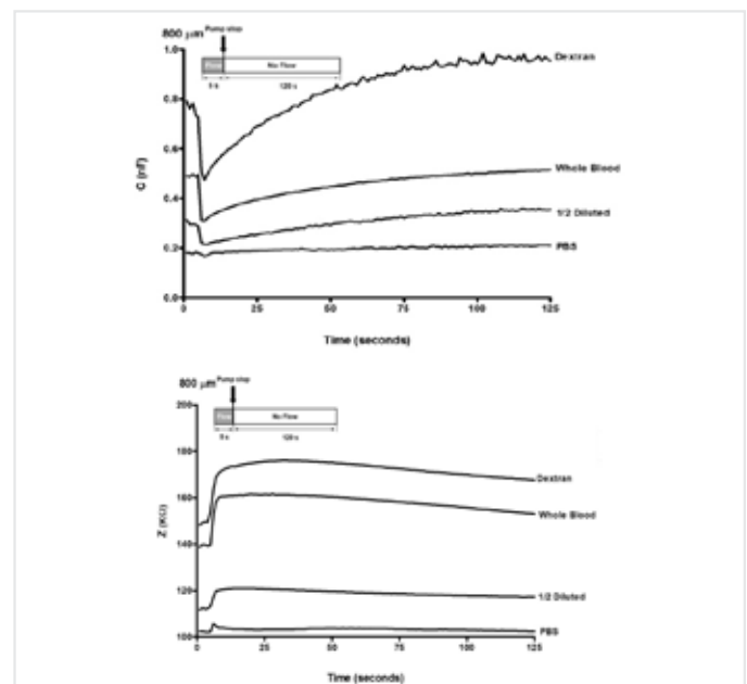
Figure 3. (a) Time course of series capacitance (C) and (b) Impedance (Z) across the glass capillary after a sudden stop of flow of red blood cell suspended in dextran, whole blood and 1/2 diluted plasma. Capacitance and impedance were monitored at 100 KHz frequency PBS: Phosphate-buffered saline
